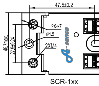
SCR-1xx
